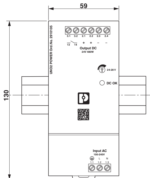
Figure 6 Device dimensions (dimensions in mm)
