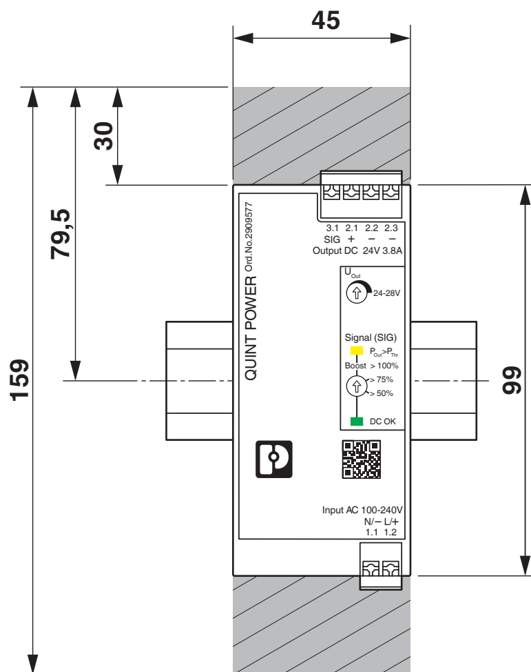
Dimensional drawing
