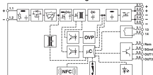
Block diagram
